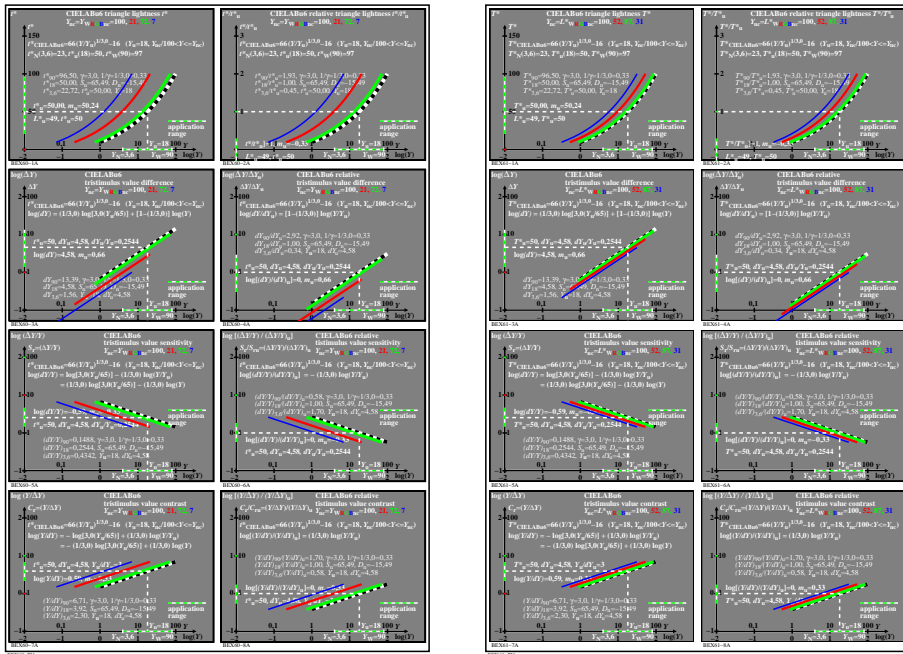
TUB-test chart BEX6; CIELABu6, t^* & T^* for Y/Y_u with additional data, Y_{nc} = (Y & L^*)_{WRGBnc} Absolute and relative lightness, sensitivity and contrast, S_u = 65.49, 1/\gamma = 1/3.0 = 0.33, D_u = 15.49
