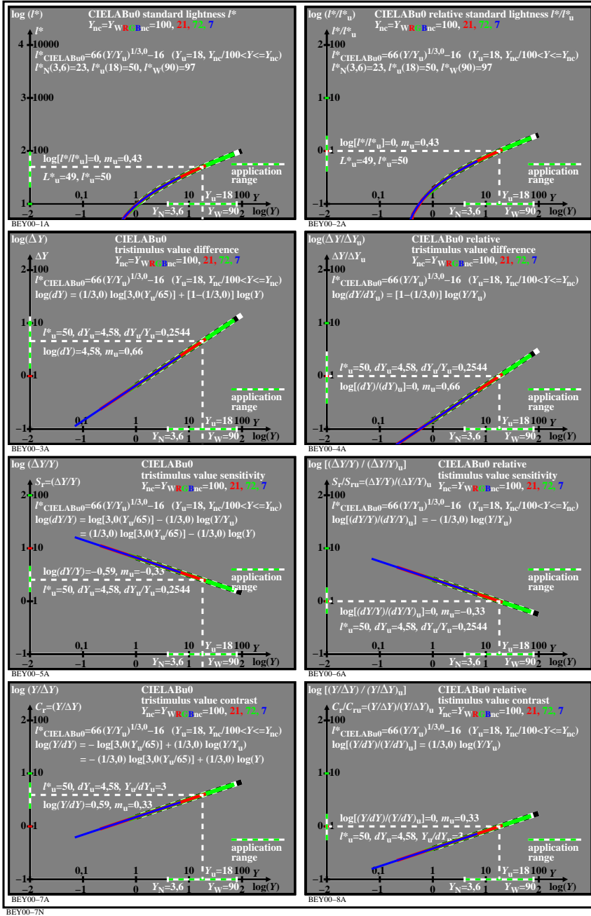
TUB-test chart BEY0; CIELABu0, l^* & L^* for Y/Y_u, Y_{nc}=(Y \cdot L^*)_{Wnc} Absolute and relative lightness, sensitivity and contrast, S_n=65,49, 1/\gamma=1/3,0=0,33, D_n=-15,49
