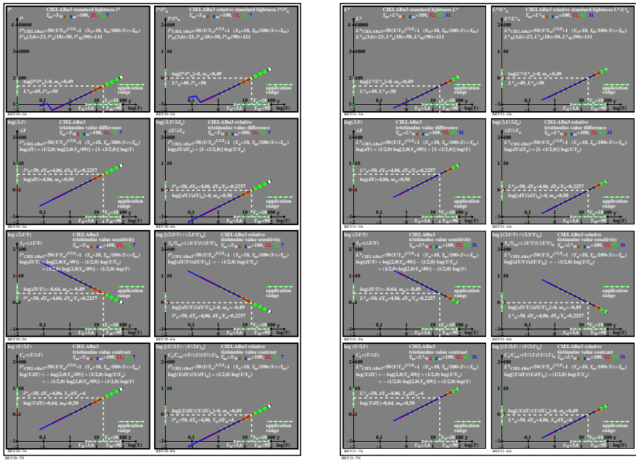
TUB-test chart BEY3; CIE LABu3, I^* & L^* for Y/Y_{nc} , Y_{nc} = (Y \cdot L^*)_{Wnc} Absolute and relative lightness, sensitivity and contrast, S_n = 49, 21, 1/\gamma = 1/2, 0 = 0.50, D_n = 0.78
