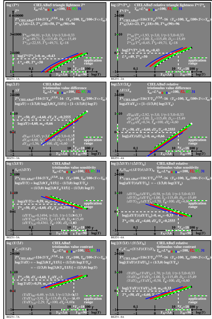
TUB-test chart BEZ5; CIELABn5, t^* & T^* for Y/Y_n with additional data, Y_{nc}=(Y \cdot L^*)WRGB_{nc} Absolute and relative lightness, sensitivity and contrast, S_n=115,49 , 1/\gamma=1/3,0=0,33 , D_n=-15,49
