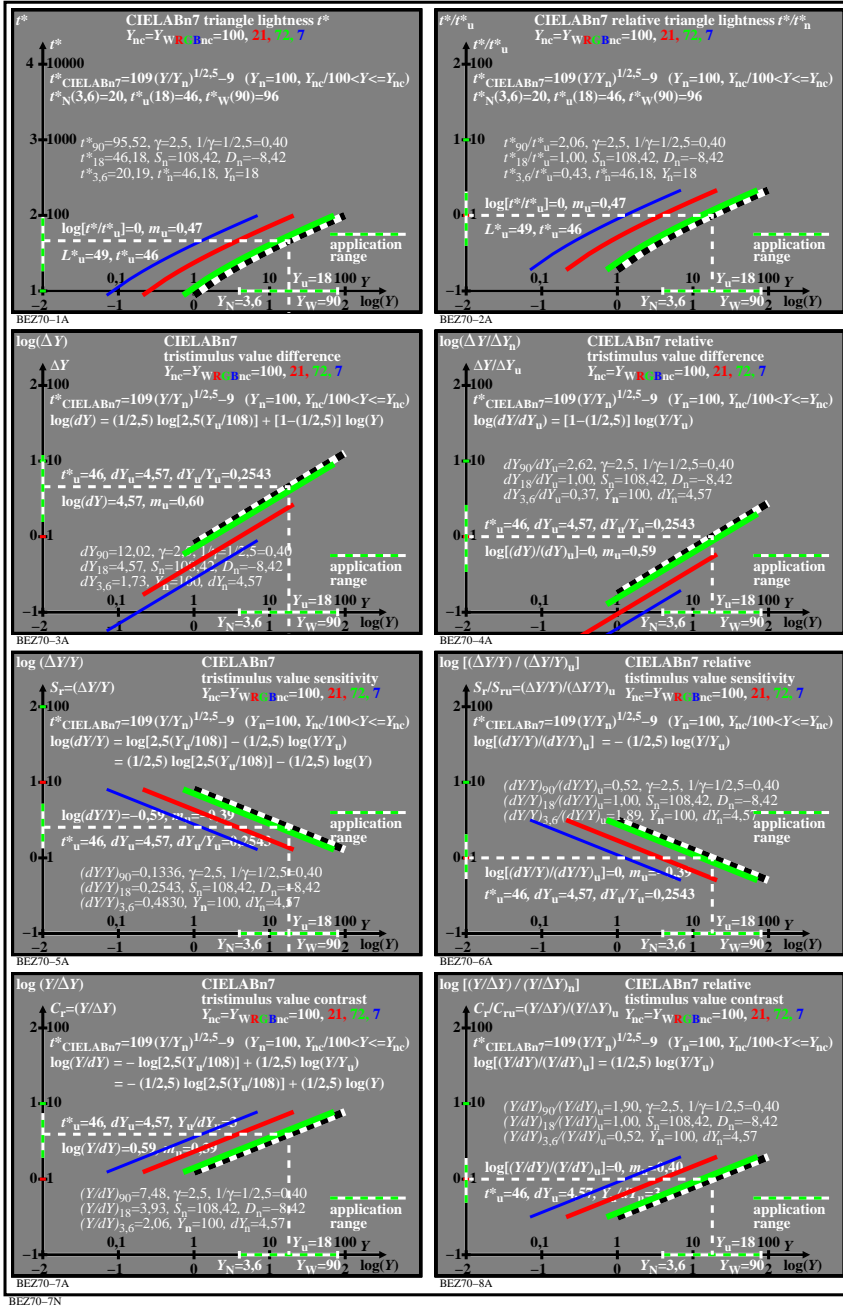
TUB-test chart BEZ7; CIELABn7, t^* & T^* for Y/Y_n with additional data, Y_{nc}=(Y \& L^*)_{WRGBnc} Absolute and relative lightness, sensitivity and contrast, S_n=108.42, 1/\gamma=1/2.5=0.40, D_n=-8.42
