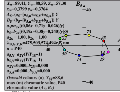
TUB-test chart CE21; CIE (x, y) and chromatic values ( A_i, B_i ) input: w/rgb/cmyk -> rgb Ostwald optimal colours for illuminant P40; diagram for illuminant P40, Y_w=88,6
