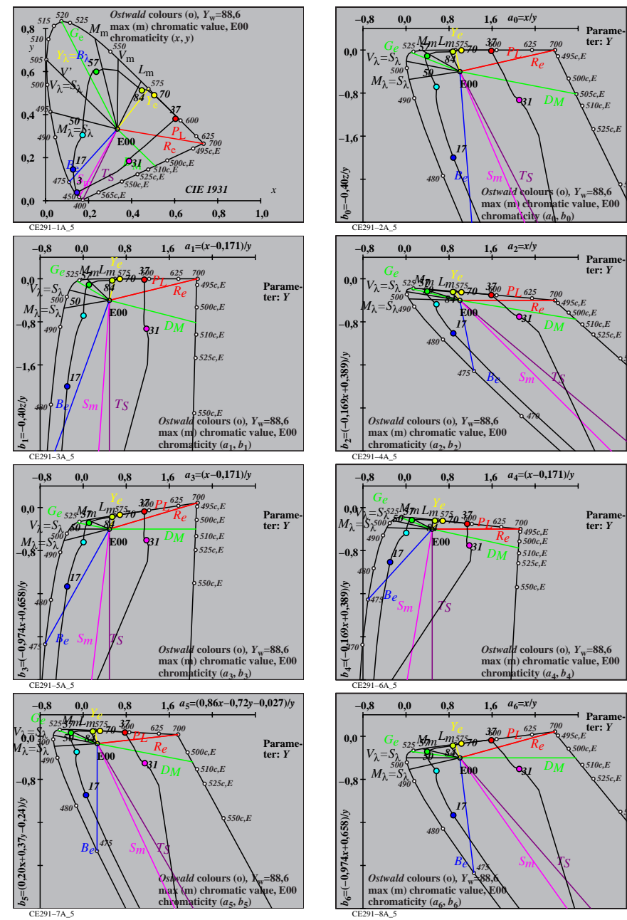
TUB-test chart CE29; CIE (x, y) and chromaticities ( a_i, b_i ) Ostwald optimal colours for illuminant E00; diagram for illuminant E00, Y_w=88,6
