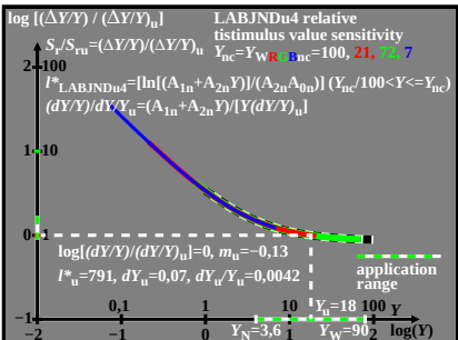
CEC40-6A
