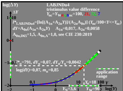
CEC40-3A
