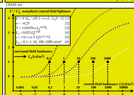
TUB-test chart CES5; Achromatic thresholds, contrast, and lightness Experimental data of Lingelbach and Richter ; Visual threshold and Weber Fechner law
