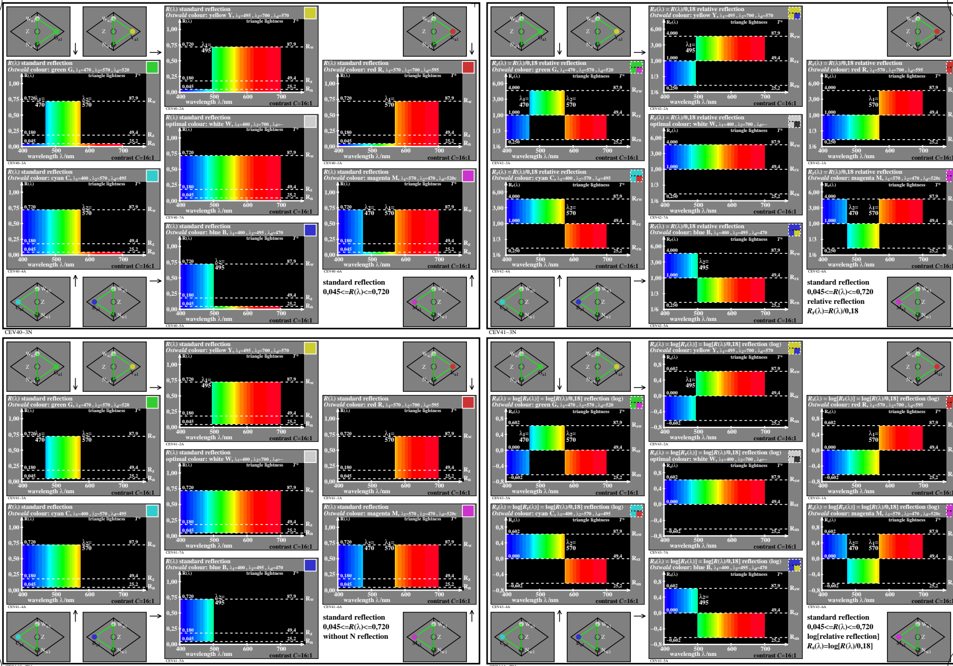
TUB-test chart CEV4; Wavelength ranges of 6 Ostwald colours, and white W Reflections R(\lambda) , R_r(\lambda) = R(\lambda)/0.18 , and R_s(\lambda) = \log[R_r(\lambda)] , triangle lightness T^* , contrast C = 16:1
