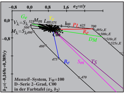
CG940-4R
