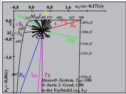
CG940-3R
