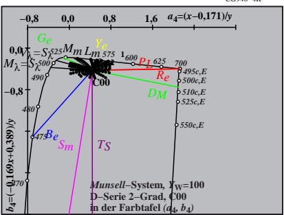
CG940-6R
