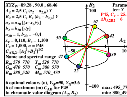
TUB-test chart DES0; TUB-Relativity model of colour vision, chromatic values of Ostwald colours for adaptation to 8 illuminants: P60, P55, P50, P45, P40, P35, P30, P25, C_r=25:1 , dh_{Ax}B_x=6
