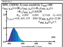
TUB-test chart EE25; XYZ-CIEF_02-degree colorimetry Cone sensitivity, and spectral tristimulus values for CIE illuminant E00, linear data
