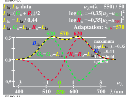
TUB-test chart EE49; Relative elementary colour vision Sensitivities \log[LMS-R17\_M5] and combinations; threshold t_a=0,00 (left) and 0,03 (right)
