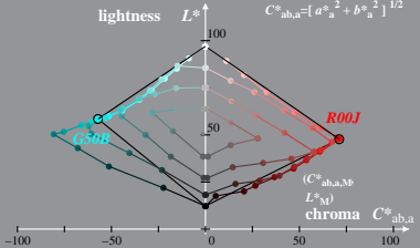
HE800-1A, 1; cfl=0.90; nt=0.18; nx=1.0
