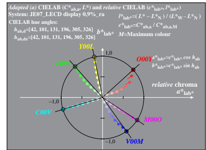
JE07-7A: Measurement: JE07_LECD display 0,9%_ra.LUT.DAT, 243 colours, 100101, Separation ob^* , adapted1/8
