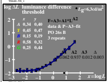
TUB-test chart TE64; threshold data Avramopoulos (89) tp=26s, 4 observers, 3 repeats, P-A3-fit, 6.3cd/m²
