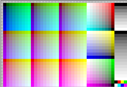
eec40-1A, gamma g_s=1,140 , g_p=0,475 , C_{YP1}
