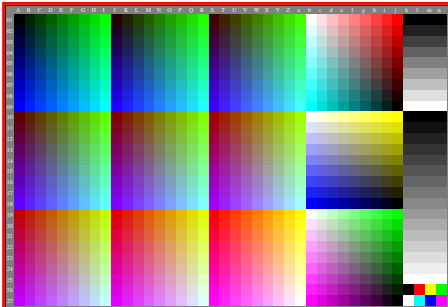
egc50-1A, Gamma g_R=2,400 , g_P=1,000 , C_{YPS}=C_{YNS}
