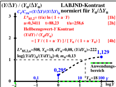
fgm60-8A
