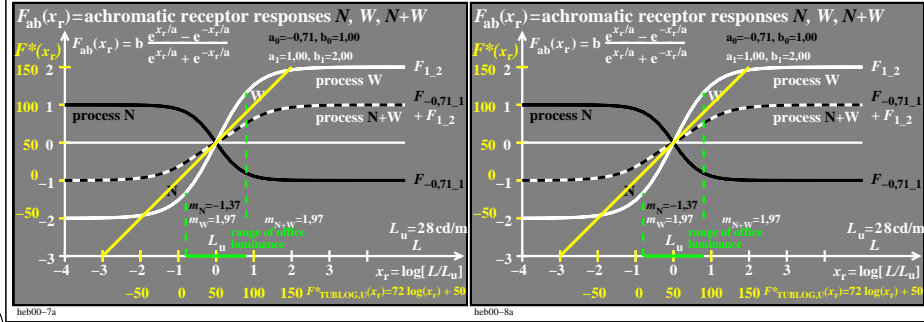
TUB-test chart heb0; Model of response functions F_{ab}(x_r) , processes N, W, N+W Tangens hyperbolicus \tanh(x_r) and modified with e^{\pm x_r/a} and 10^{\pm x_r/a} ; a = -0,71 \ \& \ 1,00 ; a' = a \ln(10)
