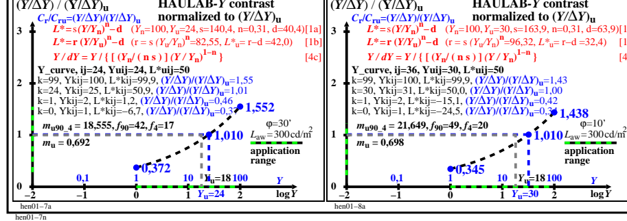
TUB-test chart hen0; HAULAB, sample-viewing angles 120' to 10', Haubner (1980) & data lin[lighness L^* , threshold \Delta Y , sensitivity \Delta Y / Y , contrast Y / \Delta Y , normalized for grey U]
