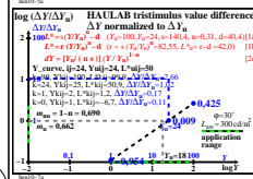
TUB-test chart hen1; HAULAB, sample-viewing angles 120° to 10°, Hubner (1980) & data log[lightness L^* , threshold \Delta Y , sensitivity \Delta Y/Y , contrast Y/\Delta Y , normalized for grey U]
