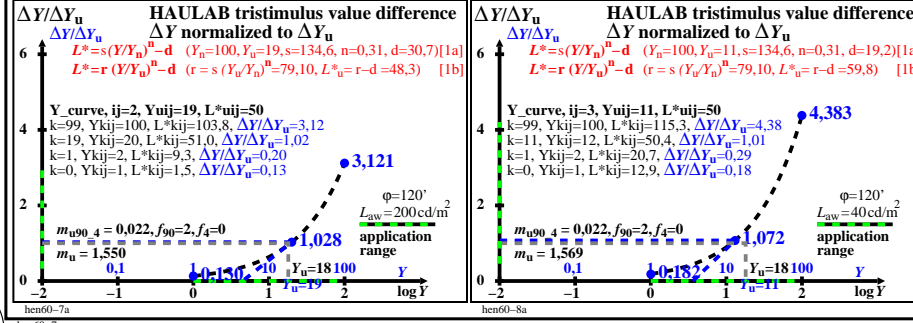
TUB-test chart hen6; HAULAB, adaptation W Lwu=300, 1000, 200, 40, Haubner (1980) & data lin[lighness L*, threshold ΔY, sensitivity ΔY / Y, contrast Y / ΔY, normalized for grey U]
