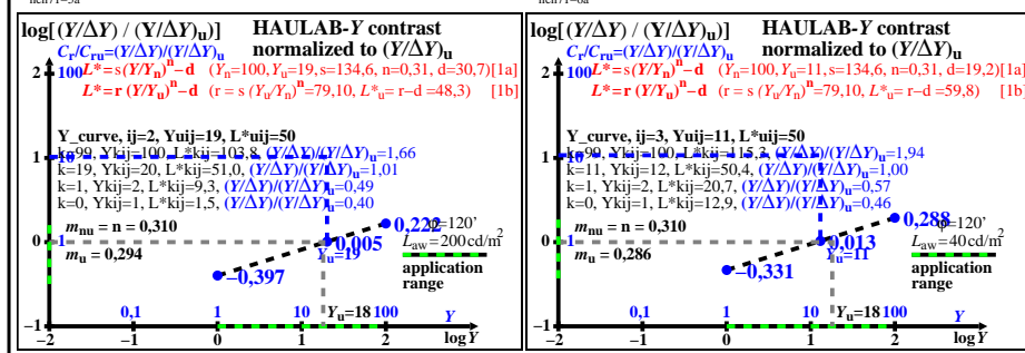
TUB-test chart hen7; HAULAB, adaptation W Lwu=300, 1000, 200, 40, Haubner (1980) & data log[lightness L*, threshold ΔY, sensitivity ΔY / Y, contrast Y / ΔY, normalized for grey U]
