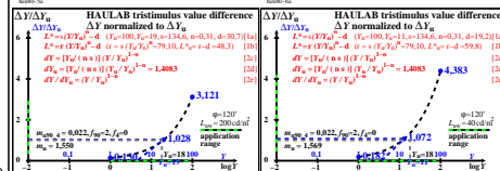
TUB-test chart hen8; HAULAB, adaptation W Lw=300, 1000, 200, 40, Haubner (1980) & equations lin[lightness L*, threshold ΔY, sensitivity ΔY/Y, contrast Y/ΔY, normalized for grey U]
