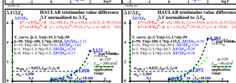
TUB-test chart heo6; HAULAB, adaptation W Lwu=300, 1000, 200, 40, Haubner (1980) & data lin[lightness L*, threshold ΔY, sensitivity ΔY/Y, contrast Y/ΔY, normalized for grey U]
