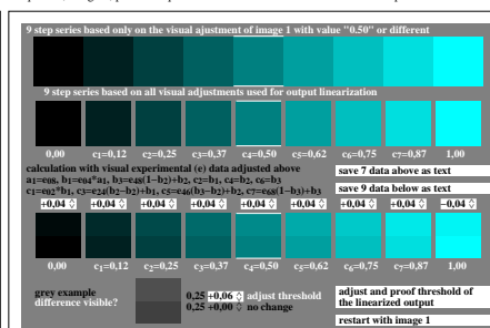
heq10-8a, image 4, adjust visual threshold (+0.047) of 9 steps; all equal?
