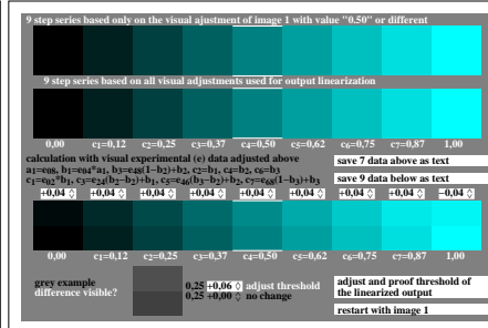
heq10-4a, image 4, adjust visual threshold (+0.047) of 9 steps; all equal?
