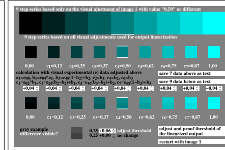
heq11-4a, image 4, adjust visual threshold (+0.047) of 9 steps; all equal?
