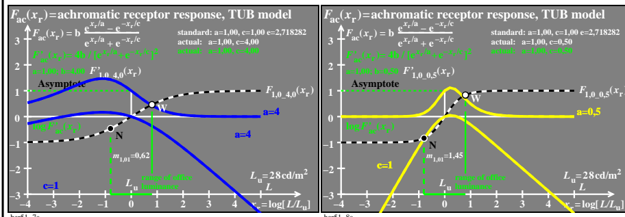
TUB-test chart her5; Model of normalized response function F_{ab}(x_r) and derivation F'_{ab}(x_r) Mathematical calculation of the derivation F'_{ab}(x_r) , of the contrast L/\Delta L , and the discrimination \Delta L
