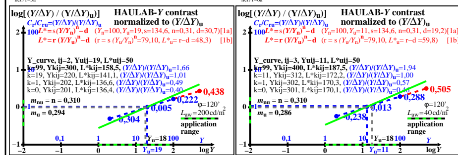
TUB-test chart het7; HAULAB, adaptation W Lwu=300, 1000, 200, 40, Haubner (1980) & data log[lightness L*, threshold ΔY, sensitivity ΔY / Y, contrast Y / ΔY, normalized for grey U], φ=120°
