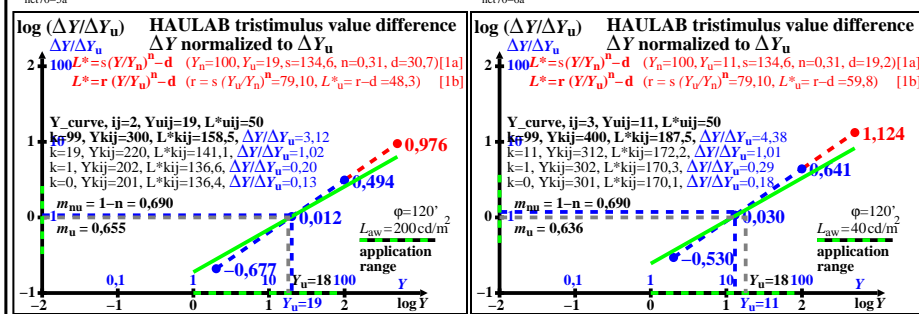
TUB-test chart het7; HAULAB, adaptation W Lwu=300, 1000, 200, 40, Haubner (1980) & data log[lightness L*, threshold ΔY, sensitivity ΔY / Y, contrast Y / ΔY, normalized for grey U], φ=120°
