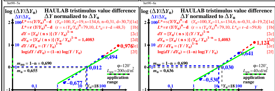
TUB-test chart het9; HAULAB, adaptation W Lwu=300, 1000, 200, 40, Haubner (1980) & equations log[lightness L*, threshold ΔY, sensitivity ΔY / Y, contrast Y / ΔY, normalized for grey U], φ=120°
