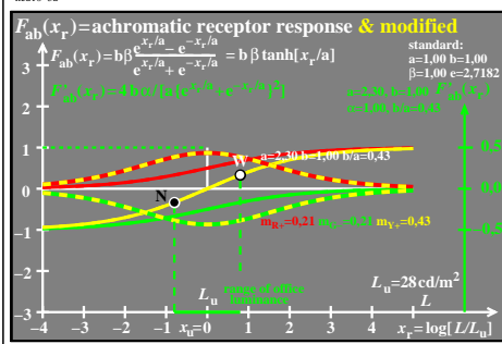
TUB-test chart heu1; TUBJND model response functions F_{ab}(x_r) , and derivation F'_{ab}(x_r) Receptor responses R_+ , G_- , Y_+ , and derivations Y_+ , Y_- (left & right), and R_+ , G_- (right)
