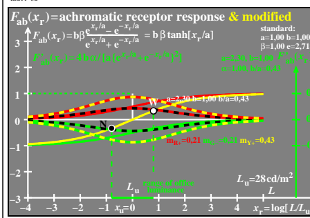
TUB-test chart heu1; TUBJND model response functions F_{ab}(x_r) , and derivation F'_{ab}(x_r) Receptor responses R_+ , G_- , Y_+ , and derivations Y_+ , Y_- (left & right), and R_+ , G_- (right)
