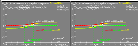
TUB-test chart hev0; TUBJND model response functions F_{ab}(x_r) , and derivation F'_{ab}(x_r) Receptor responses R+, G-, Y+ (left), and derivations R+, G-, Y- (right) for different parameters a,b
