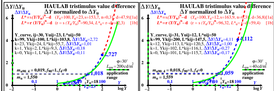
TUB-test chart hev6; HAULAB, adaptation W Lwu=300, 1000, 200, 40, Haubner (1980) & data lin[lighness L*, threshold delta Y, sensitivity delta Y / Y, contrast Y / delta Y, normalized for grey U], phi=30'
