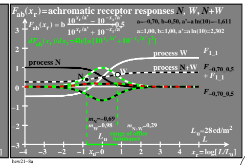
TUB-test chart hew2; Model responses F_{ab}(x_r) , processes N ( -1 \leq a \leq -0.7, b=0.5 ), W ( a=b=1 ), N+W, and derivations Tangens hyperbolicus \tanh(x_r) and modified with e^{\pm x_r/a} and 10^{\pm x_r/a} ; a'=a \ln(10) ; (+0,5)-shift
