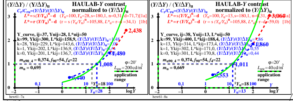
TUB-test chart hew6; HAULAB, adaptation W Lwu=300, 1000, 200, 40, Haubner (1980) & data lin[lighness L*, threshold delta Y, sensitivity delta Y / Y, contrast Y / delta Y, normalized for grey U], phi=20'
