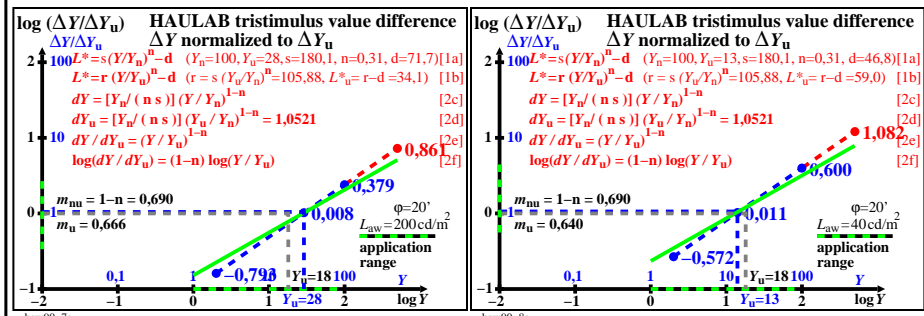
TUB-test chart hew9; HAULAB, adaptation W Lw=300, 1000, 200, 40, Haubner (1980) & equations log[lightness L*, threshold ΔY, sensitivity ΔY / Y, contrast Y / ΔY, normalized for grey U], φ=
