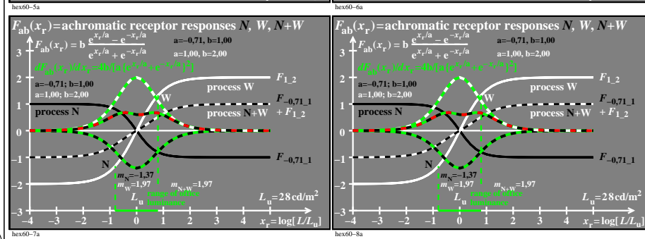
TUB-test chart hex6; Model of response functions F_{ab}(x_r) , processes N, W, N+W, and derivations Tangens hyperbolicus \tanh(x_r) and modified with e^{\pm x_r/a} and 10^{\pm x_r/a} ; a=-0.71 & 1.00 ; a' = a \ln(10)
