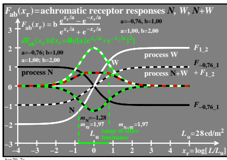
TUB-test chart hex7; Model of response functions F_{ab}(x_r) , processes N, W, N+W , and derivations Tangens hyperbolicus \tanh(x_r) and modified with e^{\pm x_r/a} and 10^{\pm x_r/a'} ; a=-0.76 & 1.00 ; a' = \ln(10)
