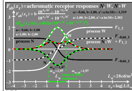
TUB-test chart hex8; Model of response functions F_{ab}(x_r) , processes N, W, N+W, and derivations Tangens hyperbolicus \tanh(x_r) and modified with e^{\pm x_r/a} and 10^{\pm x_r/a'} ; a=-0.66 & 1.00 ; a' = \ln(10)
