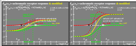
TUB-test chart hey4; TUBJND model of response functions F_{ab}(x_T) , and derivation F'_{ab}(x_T) Receptor response Y_+ , and amplitude modulations Y_+ \& R^+/G^- (left), Y_+ \& R^+/G^- (right)
