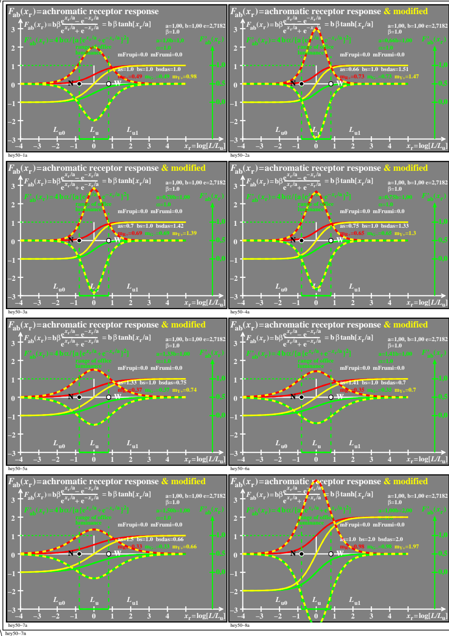
TUB-test chart hey5; TUBJND model of response functions F_{ab}(x_r) , and derivation F'_{ab}(x_r) Receptor responses R_+, G_-, Y_+ , and derivations Y_+', Y_-' (left & right), and R_+', G_-' (right)
