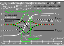
TUB-test chart hey8; Model of response functions F_{ab}(x_p) , processes N, W, N+W and derivations Tangens hyperbolicus \tanh(x_p) and modified with e^{\pm x_p/a} and 10^{\pm x_p/a} ; a = -0.66 & 1.00 ; a' = a \ln(10)
